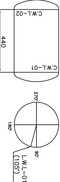
WELDING SEAM PLAN
