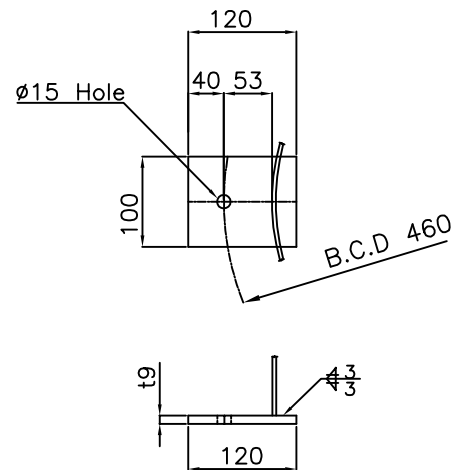
DETAIL OF BASE LATE
