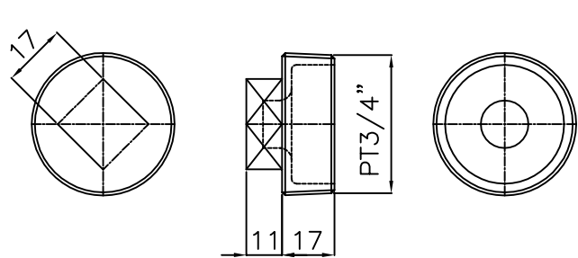
9 Inspector Hole Plug
